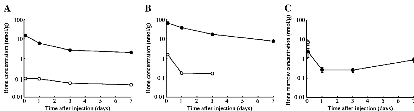
Fig. 3. Time course of bone and bone marrow concentrations of L-Asp hexapeptide-conjugated and non-conjugated quinolones. A dosage of A 27.7 \mu\text{mol/kg} of LVFX (open circle) or LVFX-D 6 (filled circle), or B 31.3 \mu\text{mol/kg} of NFLX (open circle) or NFLX-D 6 (filled circle) was intravenously injected into mice, and the concentrations in the tibia were determined at the indicated time points. The L-Asp hexapeptide-conjugated quinolones were concentrated and retained in bone at approximately 100-fold the concentrations of non-conjugated quinolones for at least 7 days after injection. C In bone marrow, LVFX was detected at 2 h after an injection of LVFX (open circle) or LVFX-D 6 (filled circle). The LVFX concentration declined to an undetectable level within 1 day after LVFX injection, whereas LVFX continued to be generated for at least 7 days after LVFX-D 6 injection. Neither NFLX nor NFLX-ga was detected in bone marrow after injection of either NFLX or NFLX-D 6 , respectively. Each point with a bar represents the mean \pm SE of four mice.
