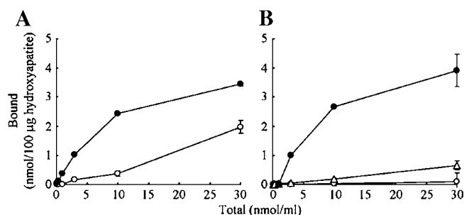
Fig. 2. Concentration-dependent binding curves of L-Asp hexapeptide-conjugated and non-conjugated quinolones to hydroxyapatite. Final concentrations of 0.1 to 30 μM of each compound, A LVFX (open circle) and LVFX-D 6 (filled circle), and B NFLX (open circle), NFLX-ga (open triangle), and NFLX-D 6 (closed circle), were incubated with 100 μg of hydroxyapatite at 37°C for 1 h. The unbound quinolone was separated from the bound quinolone by centrifugation and the concentration of unbound quinolone in the supernatant was measured. The amount of bound quinolone was calculated by subtracting the unbound from the total. L-Asp hexapeptide conjugation significantly increased the binding affinity of quinolones to hydroxyapatite. Each point with a bar represents the mean ± SE of three to six experiments.
