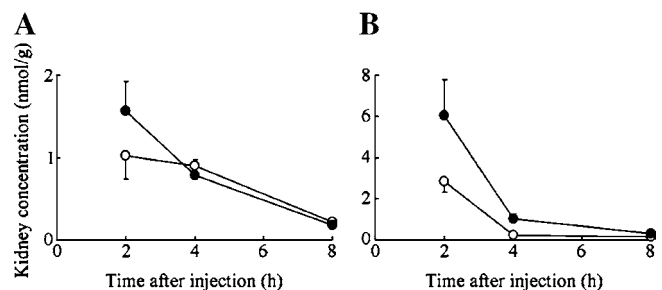
Fig. 7. Time course of kidney concentrations of L-Asp hexapeptide-conjugated and non-conjugated quinolones. A dosage of A 27.7 \mu\text{mol/kg} of LVFX (open circle) or LVFX- \text{D}_6 (filled circle), or B 31.3 \mu\text{mol/kg} of NFLX (open circle) or NFLX- \text{D}_6 (filled circle) was intravenously injected into mice, and the concentrations in kidney were determined at the indicated time points. The L-Asp hexapeptide-conjugated quinolones were concentrated in kidney at approximately two-fold the concentrations of non-conjugated quinolones at 2 h after injection. At 4 h, however, the kidney concentrations of the L-Asp hexapeptide-conjugated quinolones fell in the similar level as non-conjugated quinolones. Each point with a bar represents the mean \pm SE of four mice.
