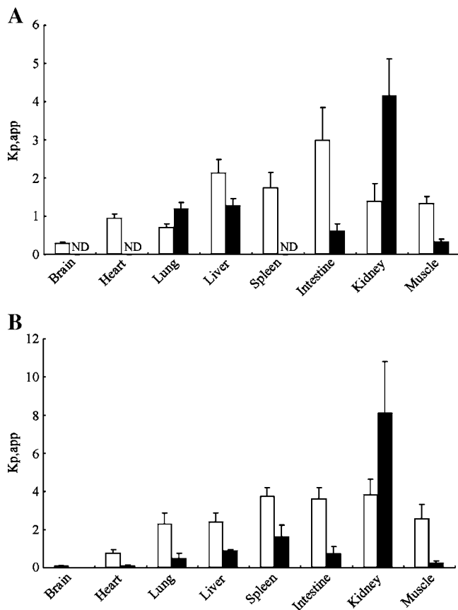
Fig. 5. Tissue distribution of L-Asp hexapeptide-conjugated and non-conjugated quinolones. A dosage of A 27.7 \mu\text{mol/kg} of LVFX (open square) or LVFX- \text{D}_6 (filled square), or B 31.3 \mu\text{mol/kg} of NFLX (open square) or NFLX- \text{D}_6 (filled square) was intravenously injected into mice, and the concentration of each compound was determined in the indicated tissues at 2 h after injection. The amounts of the L-Asp hexapeptide-conjugated quinolones were less than the amounts of the non-conjugated quinolones in most tissues, with the exception of lung and kidney tissues. The predicted products of hydrolysis (LVFX, NFLX, and NFLX-ga) were not detected in any of the soft tissues examined. Each column with a bar represents the mean \pm SE of four mice. Kp,app apparent plasma-to-tissue concentration ratios.
