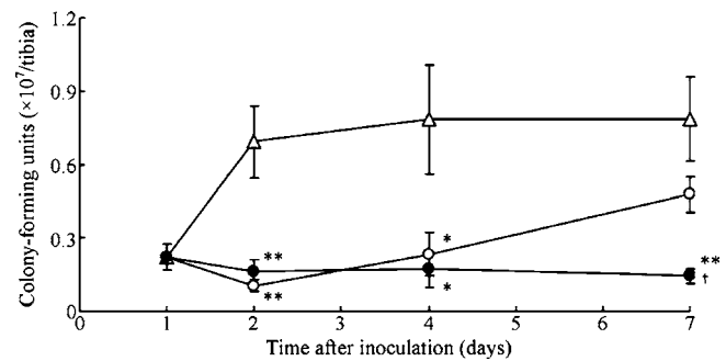
Fig. 6. Antibiotic effectiveness of LVFX and LVFX- \text{D}_6 in a mouse model of osteomyelitis. One microliter containing 10^5 cfu of S. aureus was inoculated into the tibiae of mice. The following day, LVFX (open circle) or LVFX- \text{D}_6 (filled circle) at 110.7 \mu\text{mol/kg} was intravenously injected, and the quantity of surviving S. aureus colonies was determined at the indicated time points. The cfu in untreated control mice (open square) reached a plateau 2 days post-inoculation, whereas both LVFX and LVFX- \text{D}_6 significantly suppressed the growth of S. aureus . The antibiotic efficacy of LVFX- \text{D}_6 continued for at least 6 days after injection, but the effectiveness of LVFX was temporary. Each point with a bar represents the mean \pm SE of 8–12 mice. *Significantly different from untreated control mice at p < 0.05 . **Significantly different from untreated control mice at p < 0.01 . †Significantly different from LVFX-treated mice at p < 0.01 .
