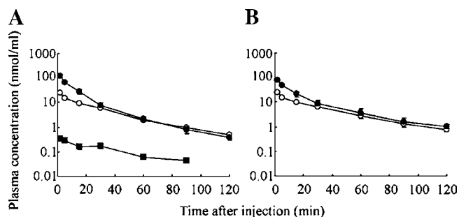
Fig. 4. Time course of plasma concentrations of L-Asp hexapeptide-conjugated and non-conjugated quinolones. A dosage of A 27.7 \mu\text{mol/kg} of LVFX (open circle) or LVFX-D 6 (filled circle), or B 31.3 \mu\text{mol/kg} of NFLX (open circle) or NFLX-D 6 (open circle) was intravenously injected into mice, and the concentrations in plasma were determined at the indicated time points. All the compounds were eliminated from the plasma in a biphasic manner. The plasma concentrations of the conjugated quinolones were two to threefold those of the non-conjugated quinolones initially after injection. However, the half-life was similar between the conjugated and non-conjugated quinolones during the elimination phase. The hydrolyzed product LVFX (filled square), which was shown in A , was detected in the plasma after LVFX-D 6 injection, and LVFX was eliminated slowly from the plasma. The predicted hydrolyzed products of NFLX-D 6 (NFLX and NFLX-ga) were not detected in the plasma after NFLX-D 6 injection. Each point with a bar represents the mean \pm SE of four mice.
