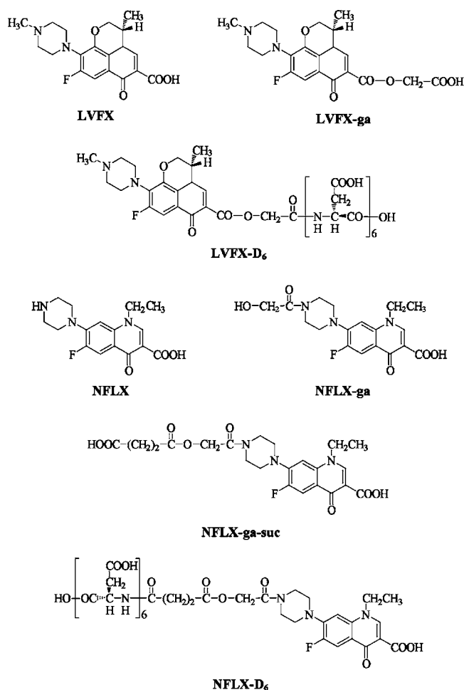
Fig. 1. Molecular structures of LVFX, glycolyl ester of LVFX ( LVFX-ga ), LVFX-D 6 , NFLX, glycolyl-NFLX ( NFLX-ga ), glycolyl-NFLX hemisuccinate ( NFLX-ga-suc ), and NFLX-D 6 .
